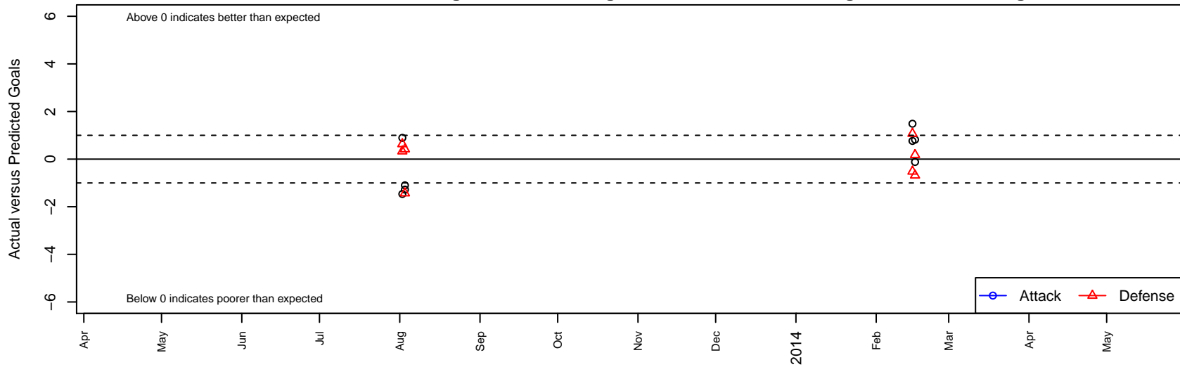
Forza FC 96 Premier B95 Dots are actual minus expected GF (blue circles) and GA (red triangles). Blue line is smoothed change in attack strength. Red is smoothed change in defense strength.
